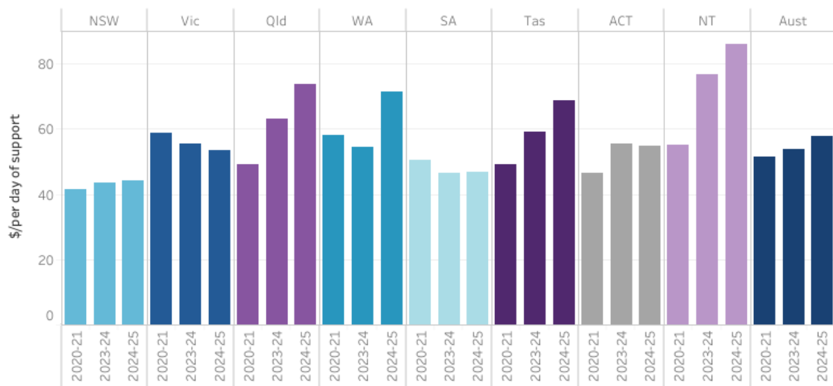
Figure 19.4 Recurrent expenditure
