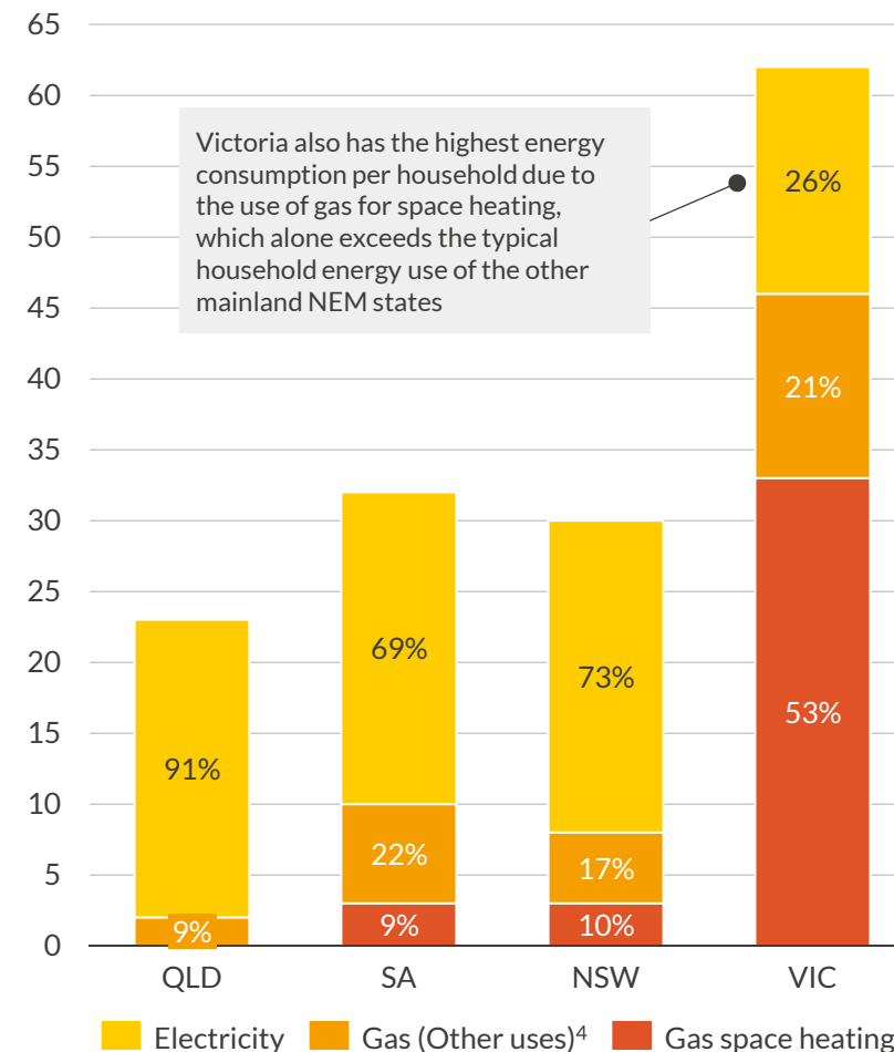
Energy use by fuel and end use per household 1
