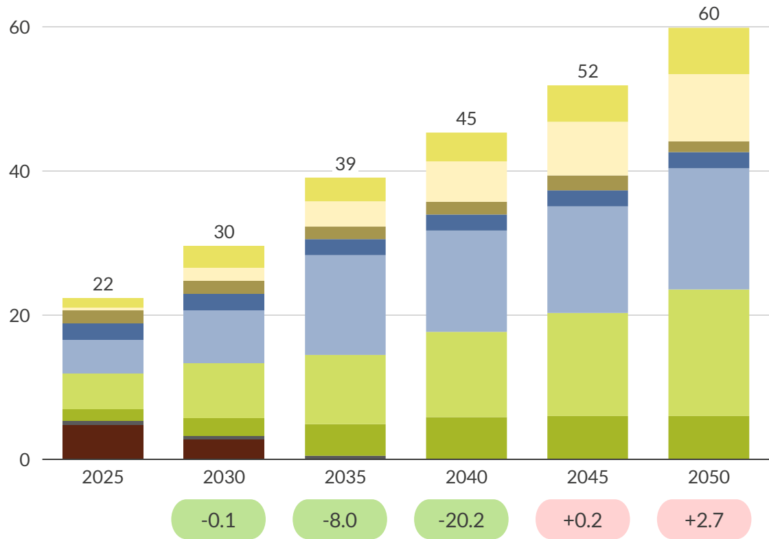
Delta from Base Case: Total 5-year CapEx for new-build utility-scale solar, wind and battery , real $A2023 bn²
