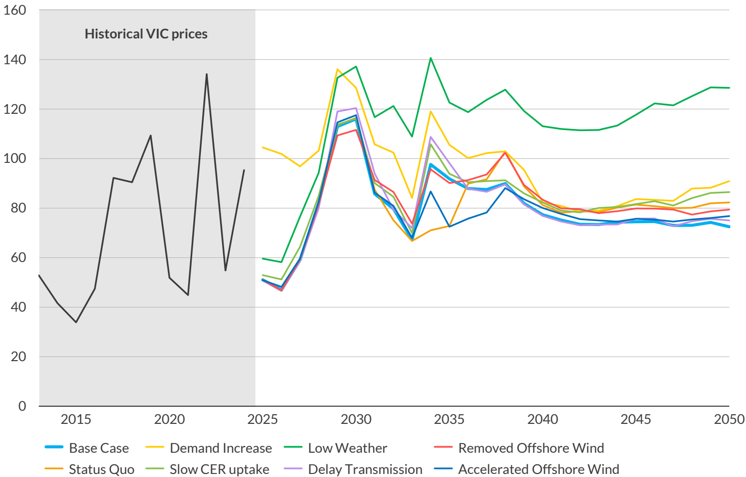
VIC Time-weighted average (TWA) price, scenario comparison $/MWh, Historical vs forecast 1
