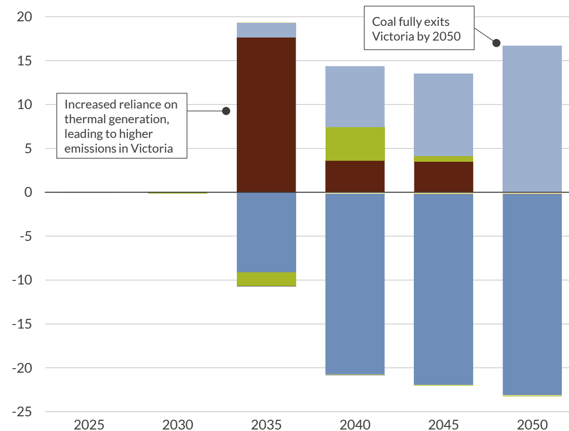
VIC Generation Delta , comparison to Base Case (BC) 3 Nameplate TWh
