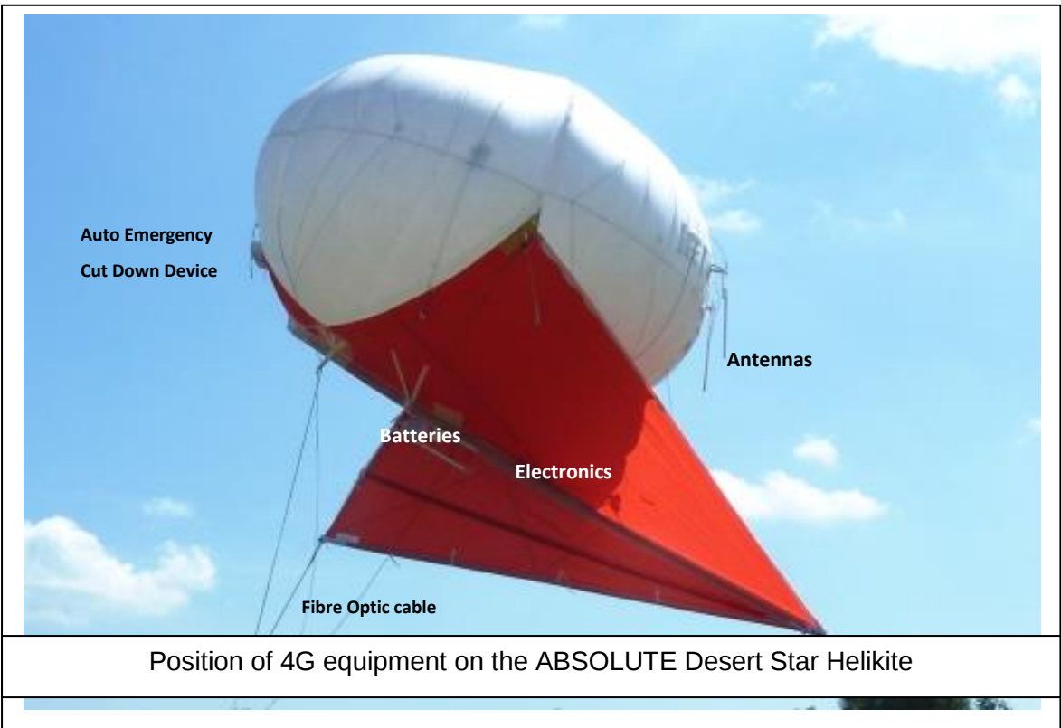
ABSOLUTE 4G 34m3 Desert Star Helikite
