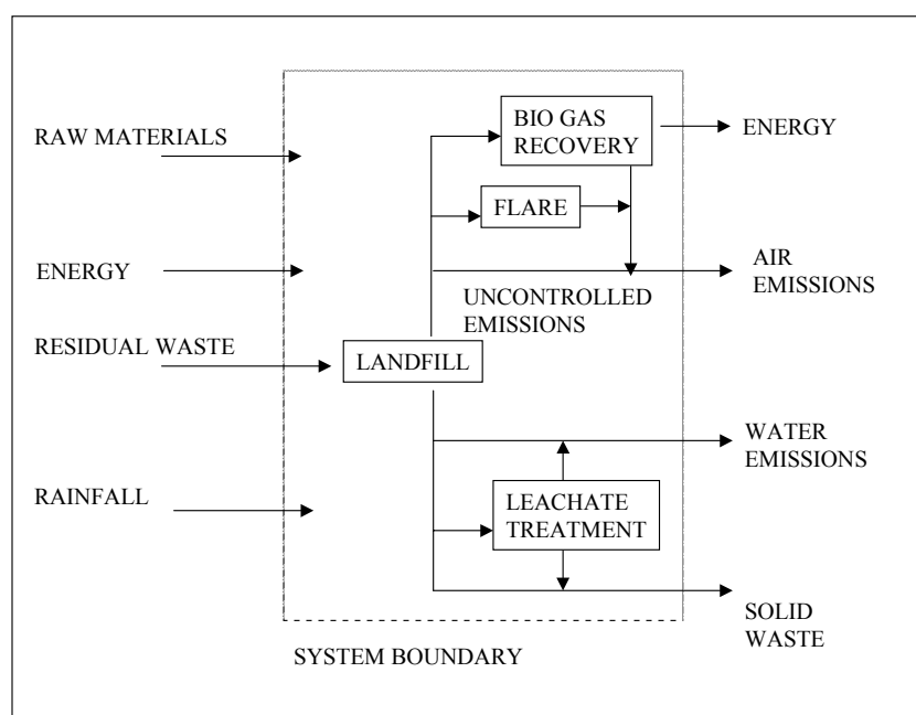
Figure 5.6: Landfill System
