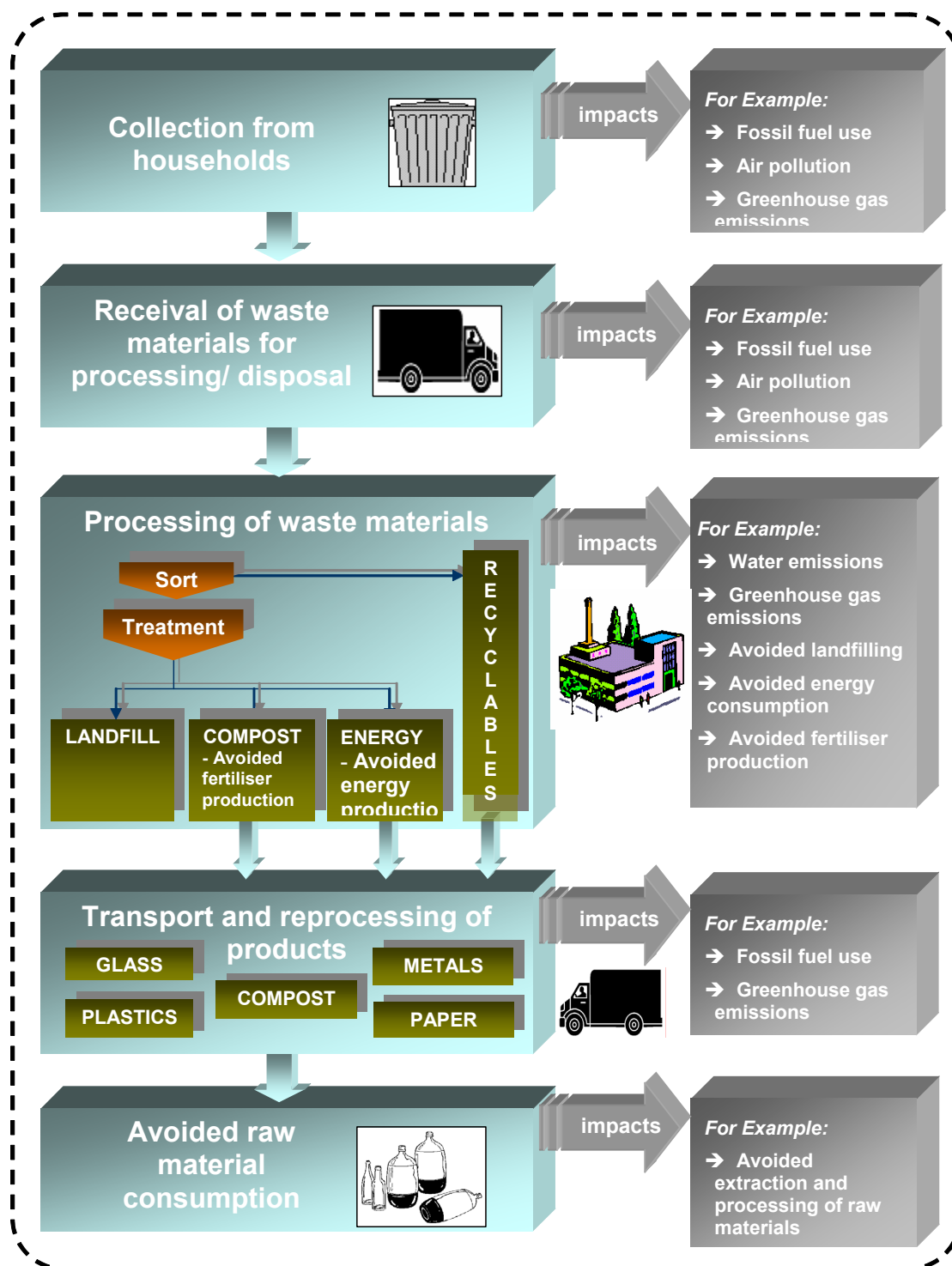
Figure 5.2: System Boundary
