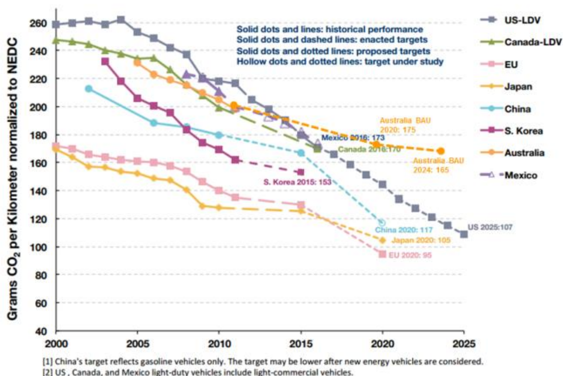
Figure 5: Comparison of new passenger vehicle fleet average emissions, actual and forecast (ICCT 2011)
