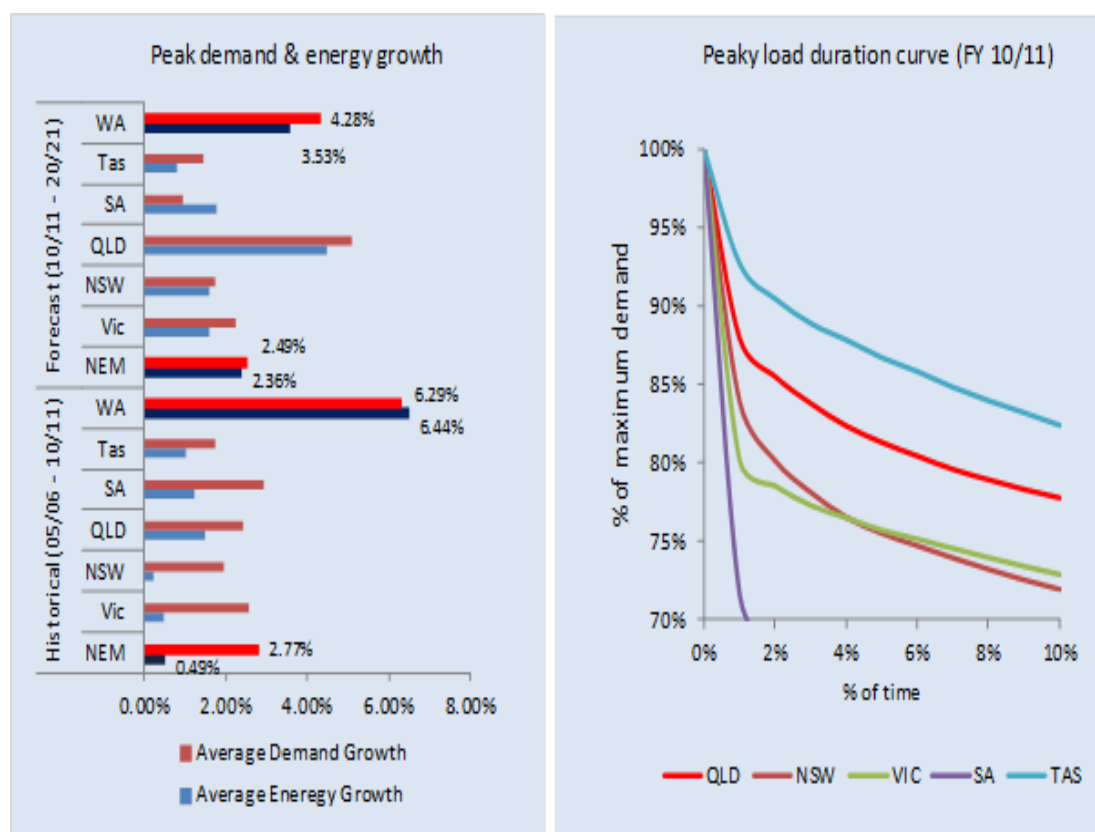
Figure 3: Peak demand and energy growth - NEM and SWIS
