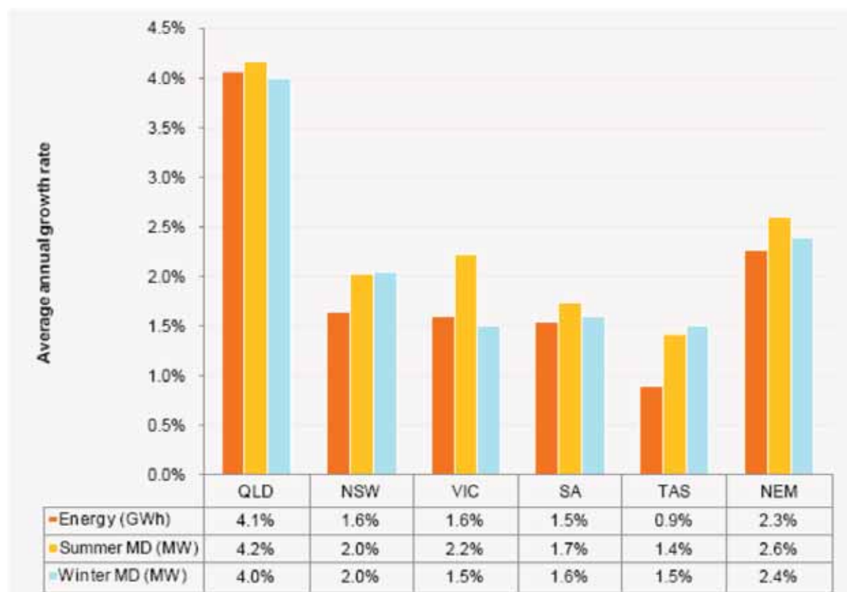
Figure 3 AEMO estimate of annual maximum demand growth and energy growth to 2020-21 6
