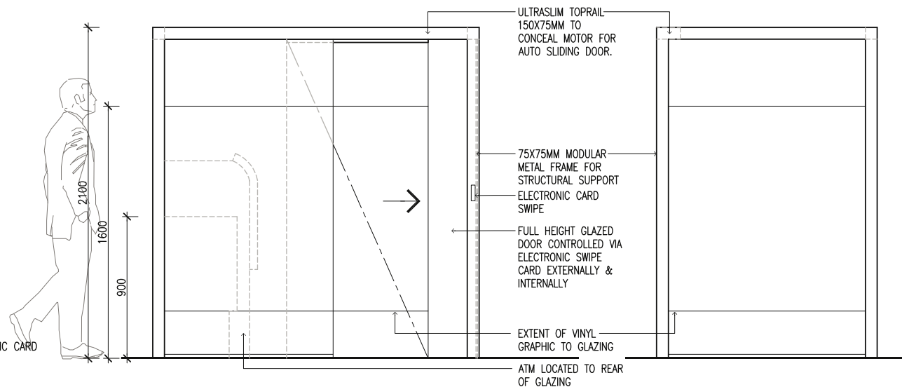
Front Elevation
